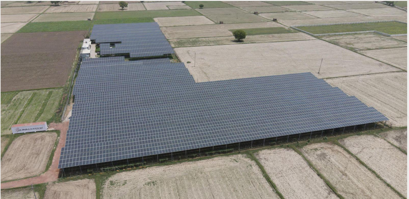
Figure 9. Aerial View of the Sunmaster Agri PV Plant Issapur Dhasa 2 - 2.5 MW
